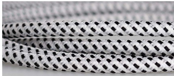
C62
